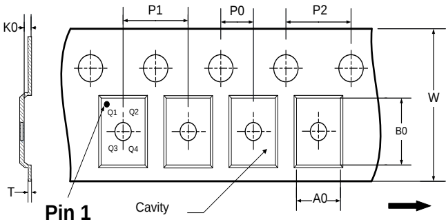
TAPE DIMENSIONS
