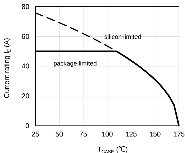
Figure 12: Current De-rating
